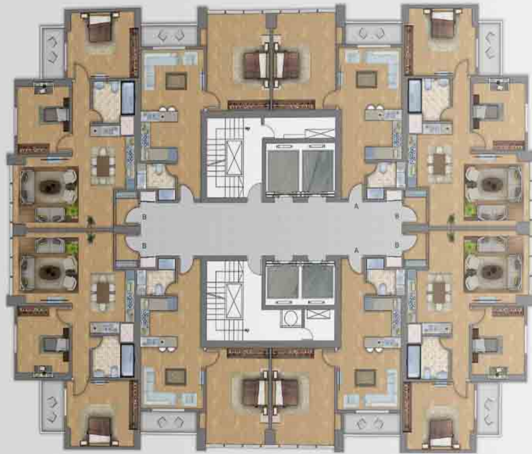
TYPICAL FLOOR PLAN 2nd - 22th
